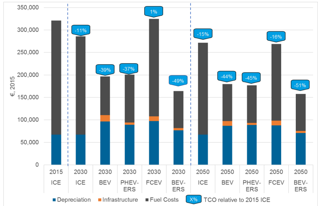
Figure 5.3 Total cost of owning and running a heavy HGV over 5 years with various powertrains in the TECH scenarios in 2030 and 2050 (€)
