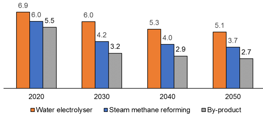
Figure 3.3 - Total costs of hydrogen production, €/kg
