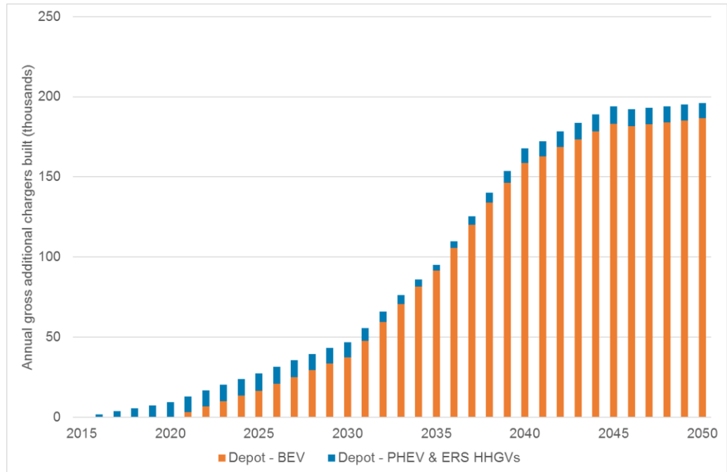
Figure 4.5: Additional depot charging points to support EV fleet in TECH BEV
