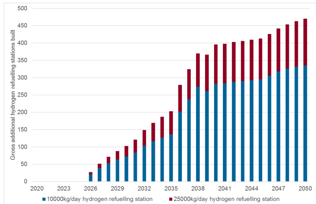
Figure 4.6: Additional HRS to support FCEV fleet in TECH FCEV
