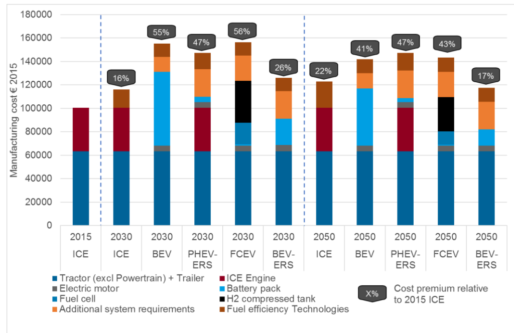
Figure 5.1 Capital cost of a new heavy HGV sized vehicle in the TECH scenarios
